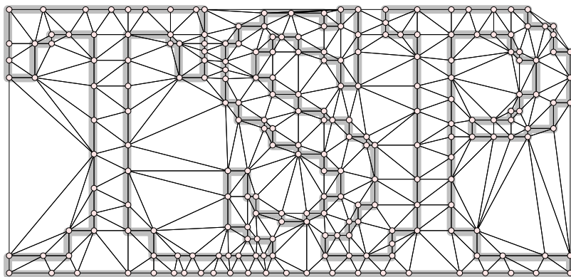
Fig. 5.8: Optimal tour of the TSP instance tsp225 on which is superimposed the Delaunay triangulation. Here, all the edges of the optimal tour are part of the triangulation
