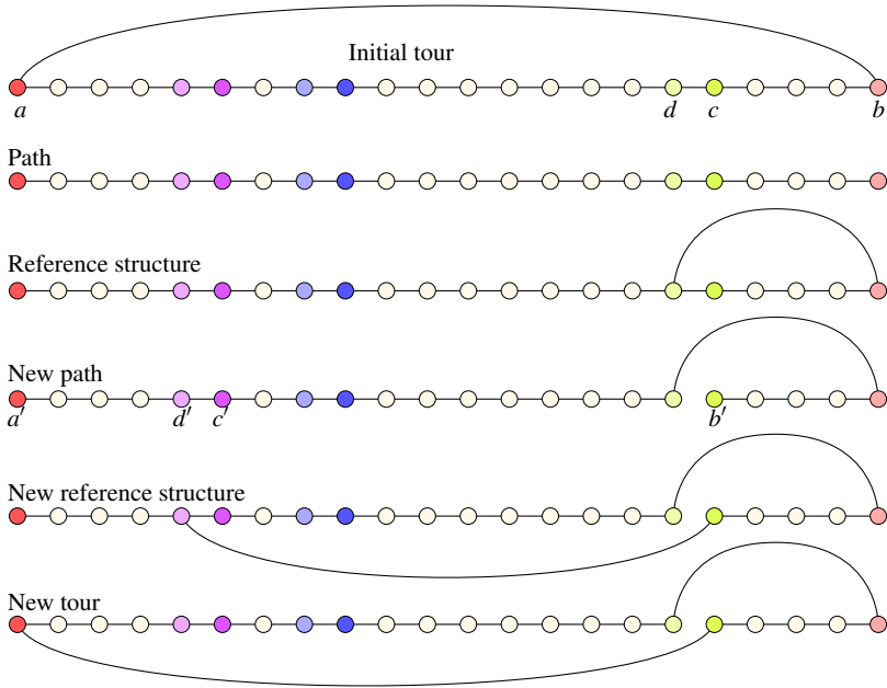
Fig. 5.10: Operating principle of an ejection chain for the TSP. Eject an edge [a,b] to get a path. Insert an edge [b,d] to get a reference structure. It can be transformed either into another reference structure, by ejection of the edge [c,d] and addition of another edge, or into a tour by ejection of [c,d] and addition of the edge [a,c]
